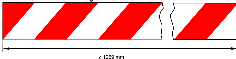
Figure A5-III Retro-reflective material marking of Class F
